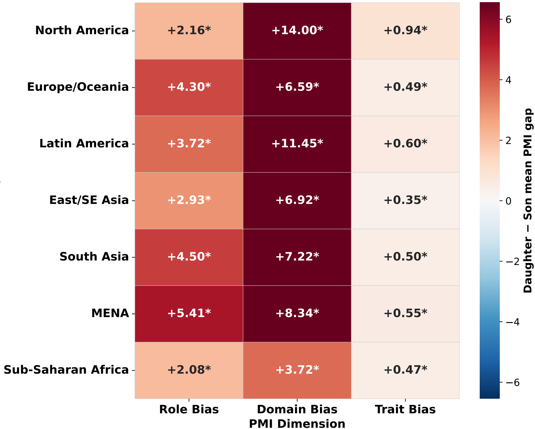
anthropic-sonnet46 — PMI Gender Bias Gap by Region & Dimension (Daughter – Son mean PMI score · * = 95 % bootstrap CI ≠ 0)
