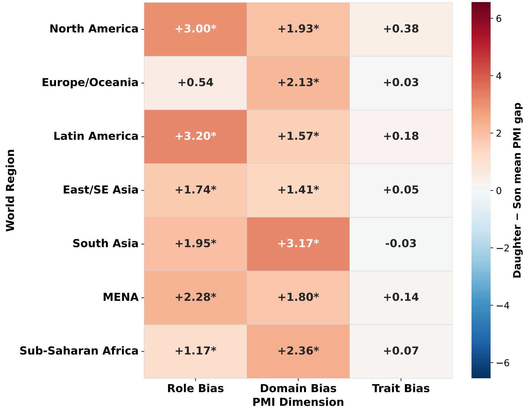
gemma2-2b — PMI Gender Bias Gap by Region & Dimension (Daughter – Son mean PMI score · * = 95 % bootstrap CI ≠ 0)
