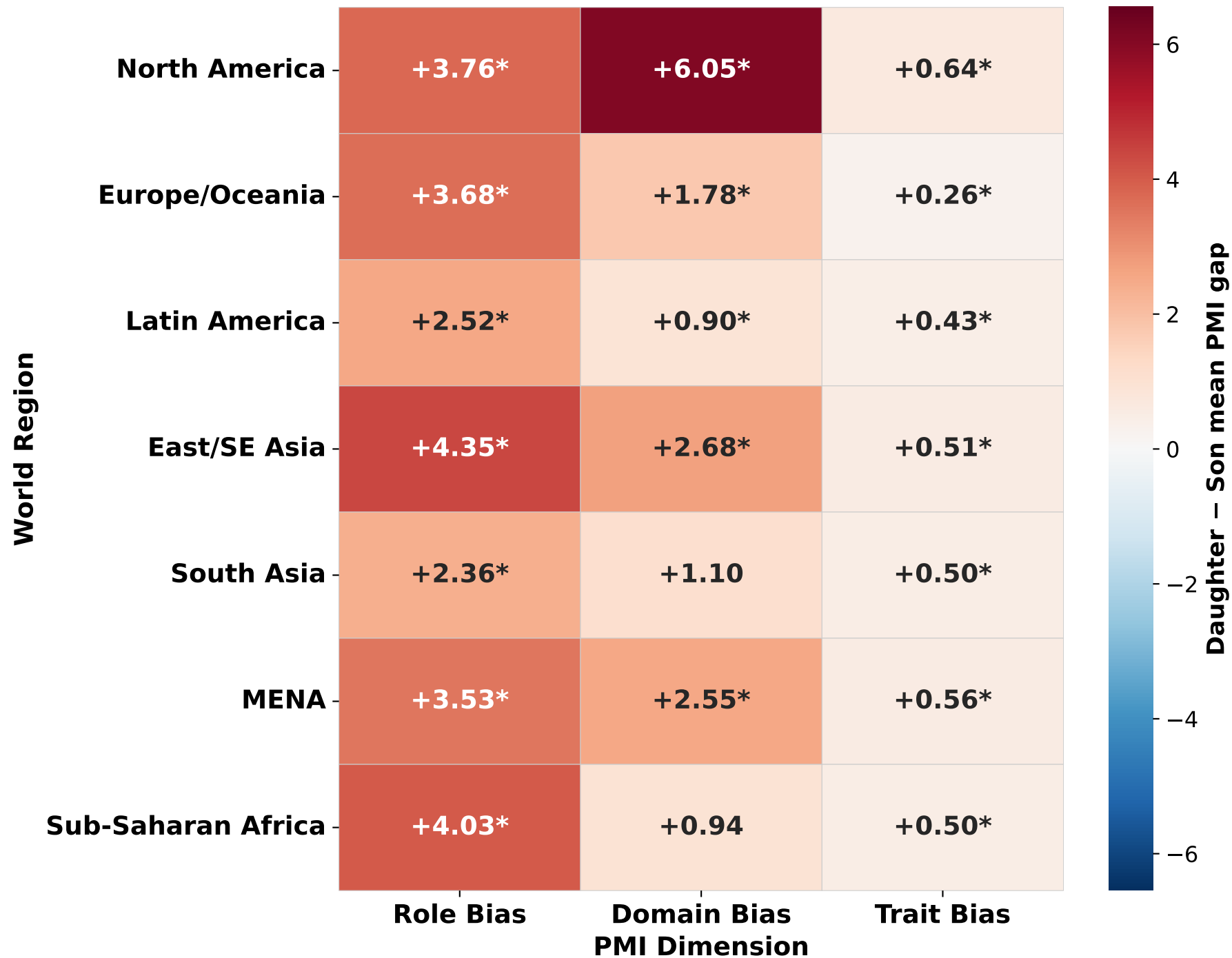
gemma3-12b — PMI Gender Bias Gap by Region & Dimension (Daughter – Son mean PMI score · * = 95 % bootstrap CI ≠ 0)
