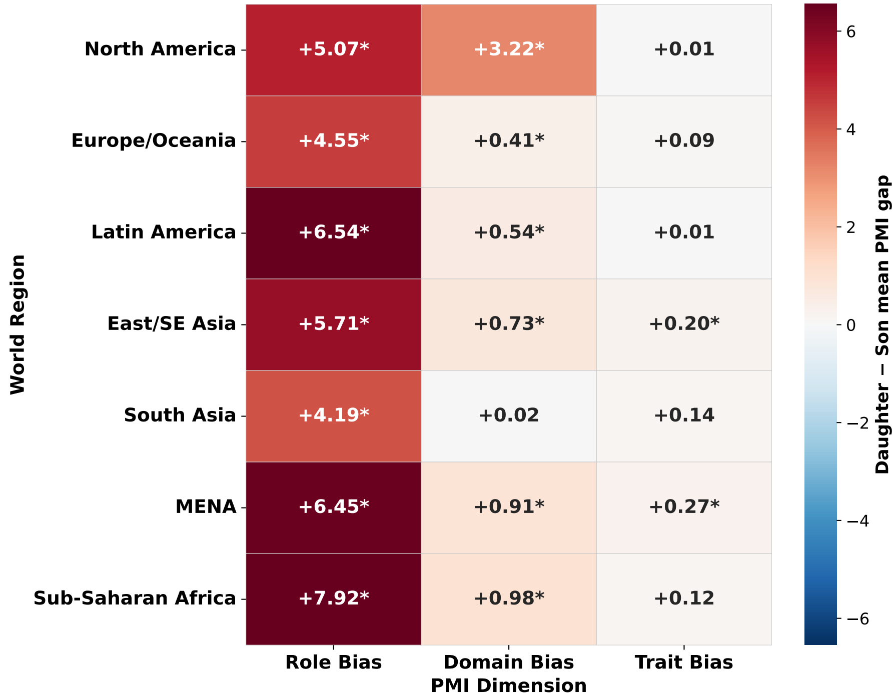
llama3-70b — PMI Gender Bias Gap by Region & Dimension (Daughter – Son mean PMI score · * = 95 % bootstrap CI ≠ 0)
