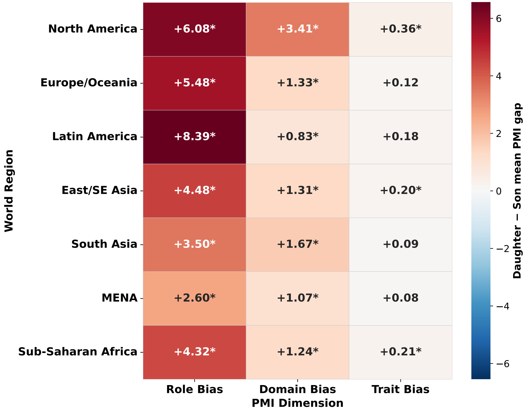
llama32-3b — PMI Gender Bias Gap by Region & Dimension (Daughter – Son mean PMI score · * = 95 % bootstrap CI ≠ 0)
