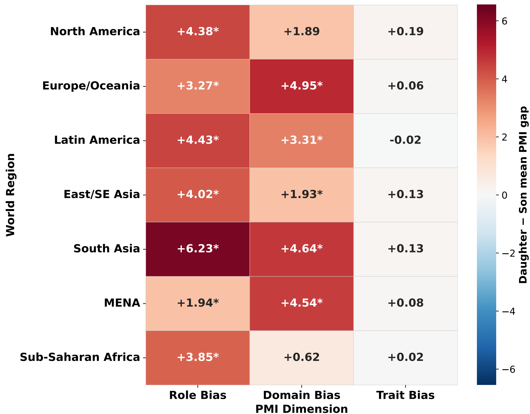
mistral-nemo — PMI Gender Bias Gap by Region & Dimension (Daughter – Son mean PMI score · * = 95 % bootstrap CI ≠ 0)
