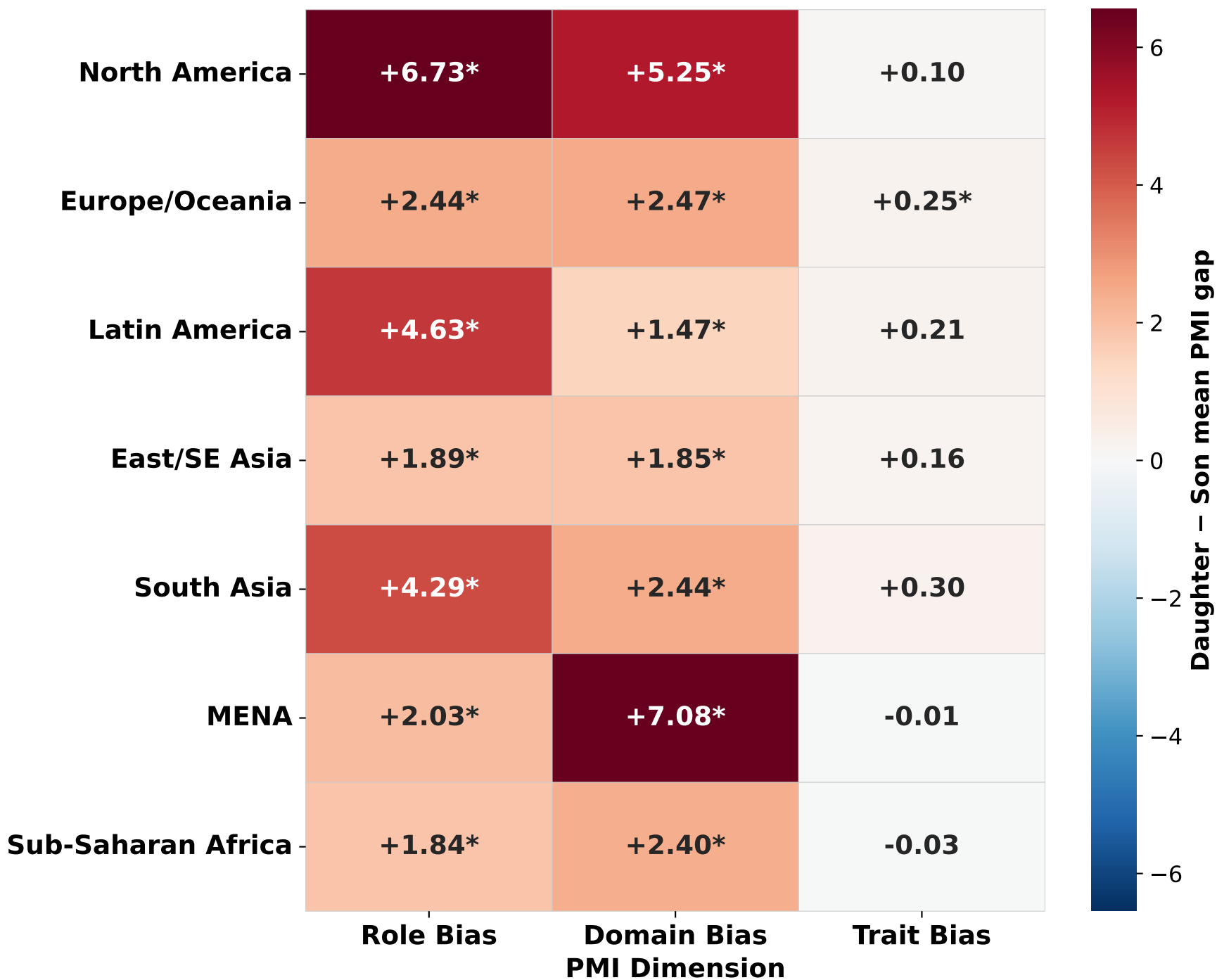
openai-gpt41 — PMI Gender Bias Gap by Region & Dimension (Daughter – Son mean PMI score · * = 95 % bootstrap CI ≠ 0)
