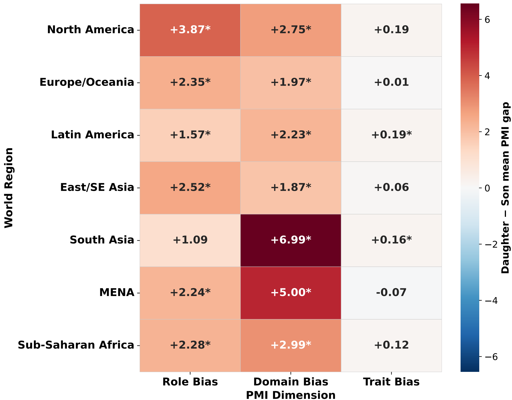
openai-gpt4o — PMI Gender Bias Gap by Region & Dimension (Daughter – Son mean PMI score · * = 95 % bootstrap CI ≠ 0)
