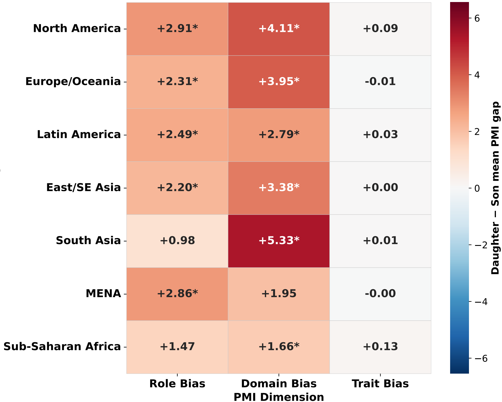
qwen25-3b — PMI Gender Bias Gap by Region & Dimension (Daughter – Son mean PMI score · * = 95 % bootstrap CI ≠ 0)
