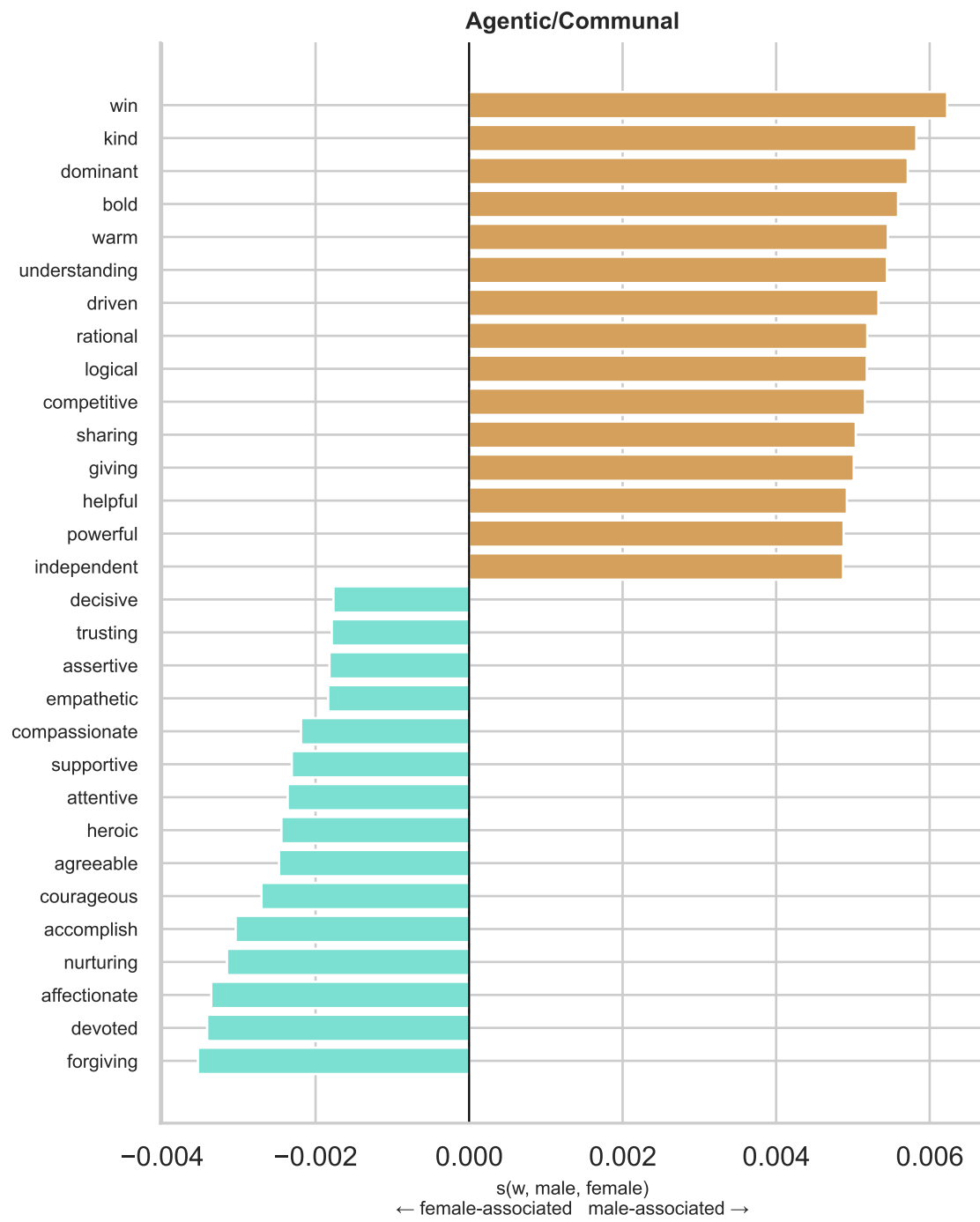
Per-Word Gender Association Scores — gemma3-12b (final layer) s(w, A, B) = \text{mean\_cos}(w, \text{male markers}) - \text{mean\_cos}(w, \text{female markers})
