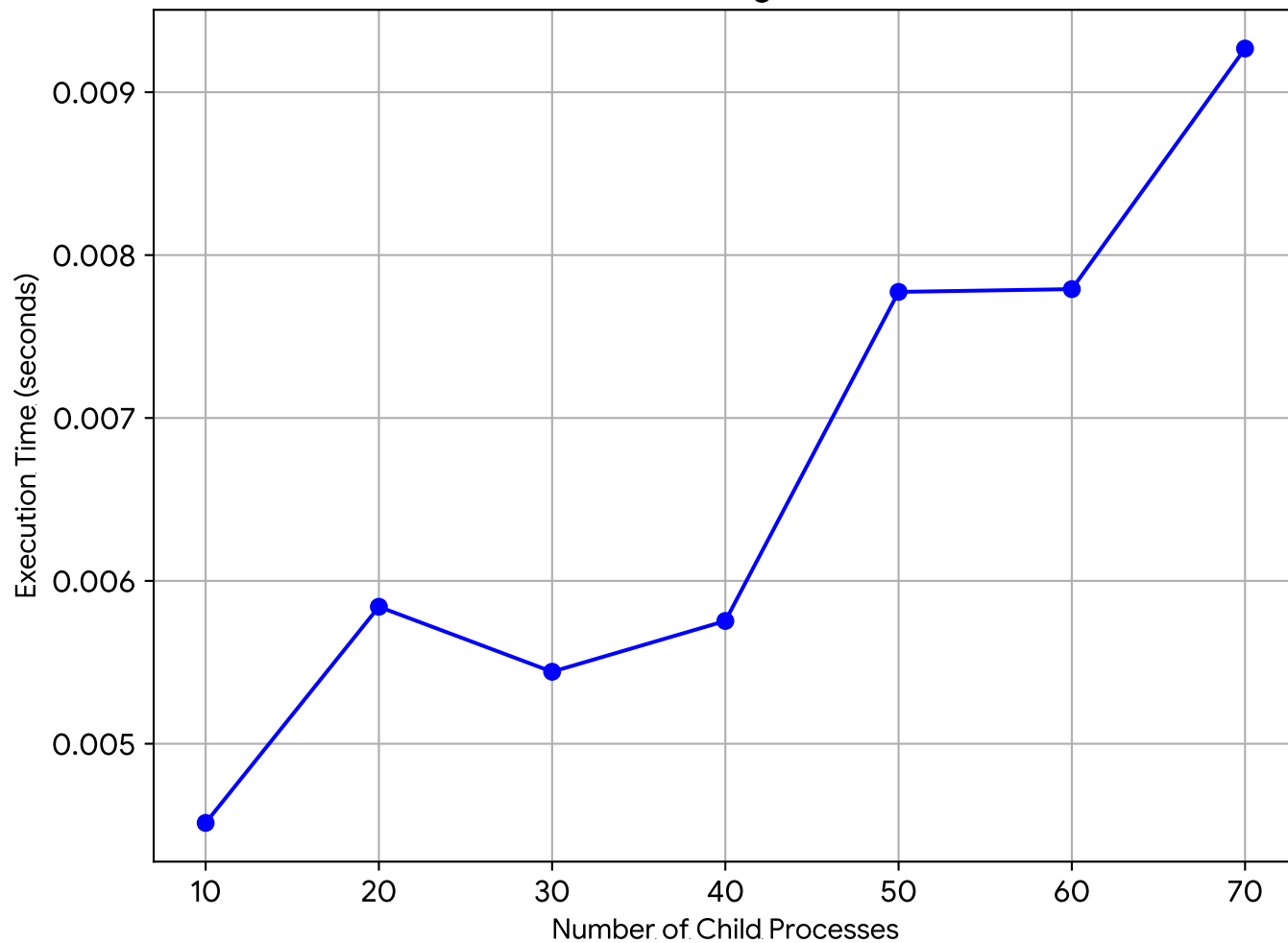
Execution Time: Range 1000 - 10000
