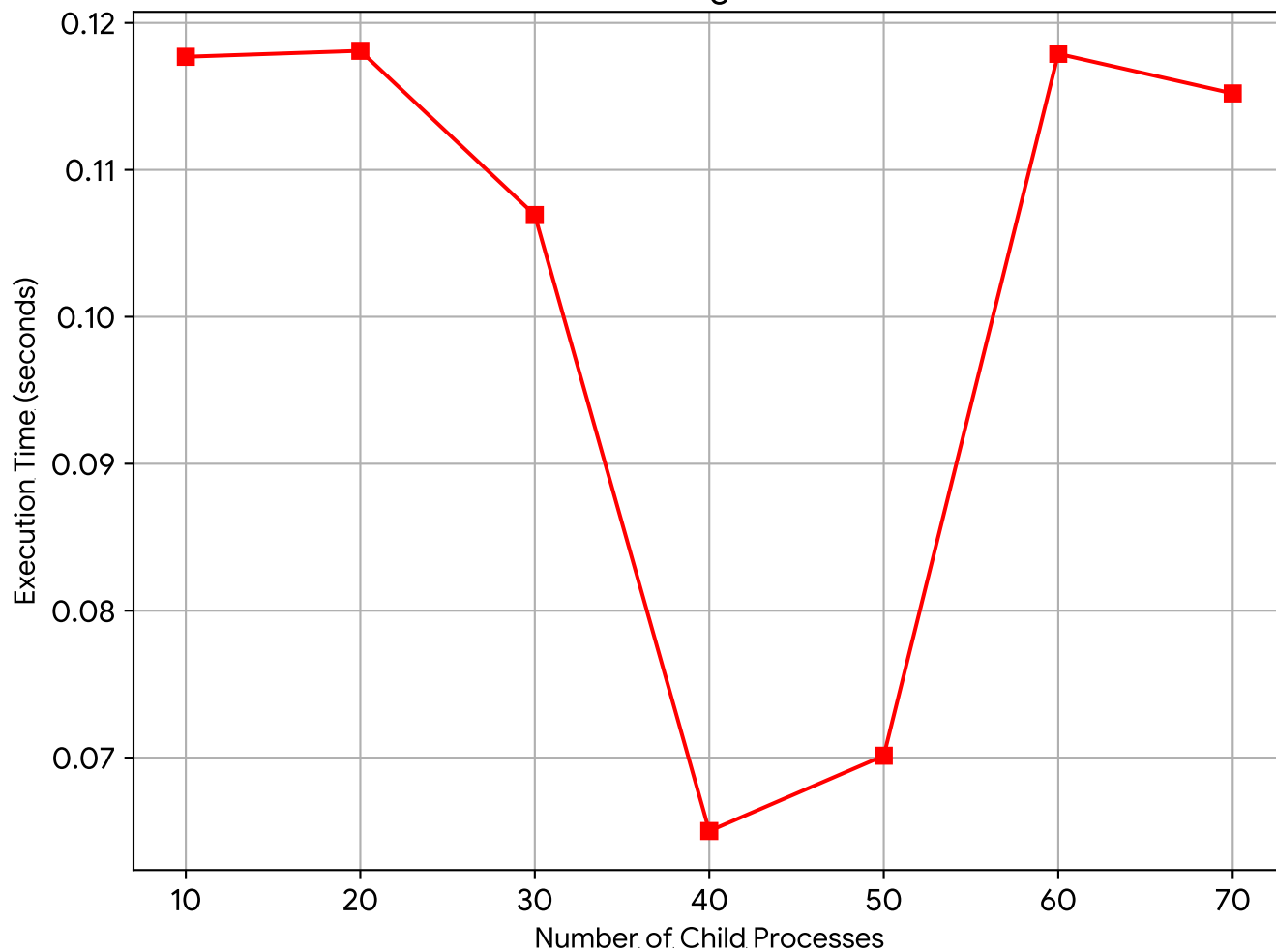
Execution Time: Range 50000 - 100000
