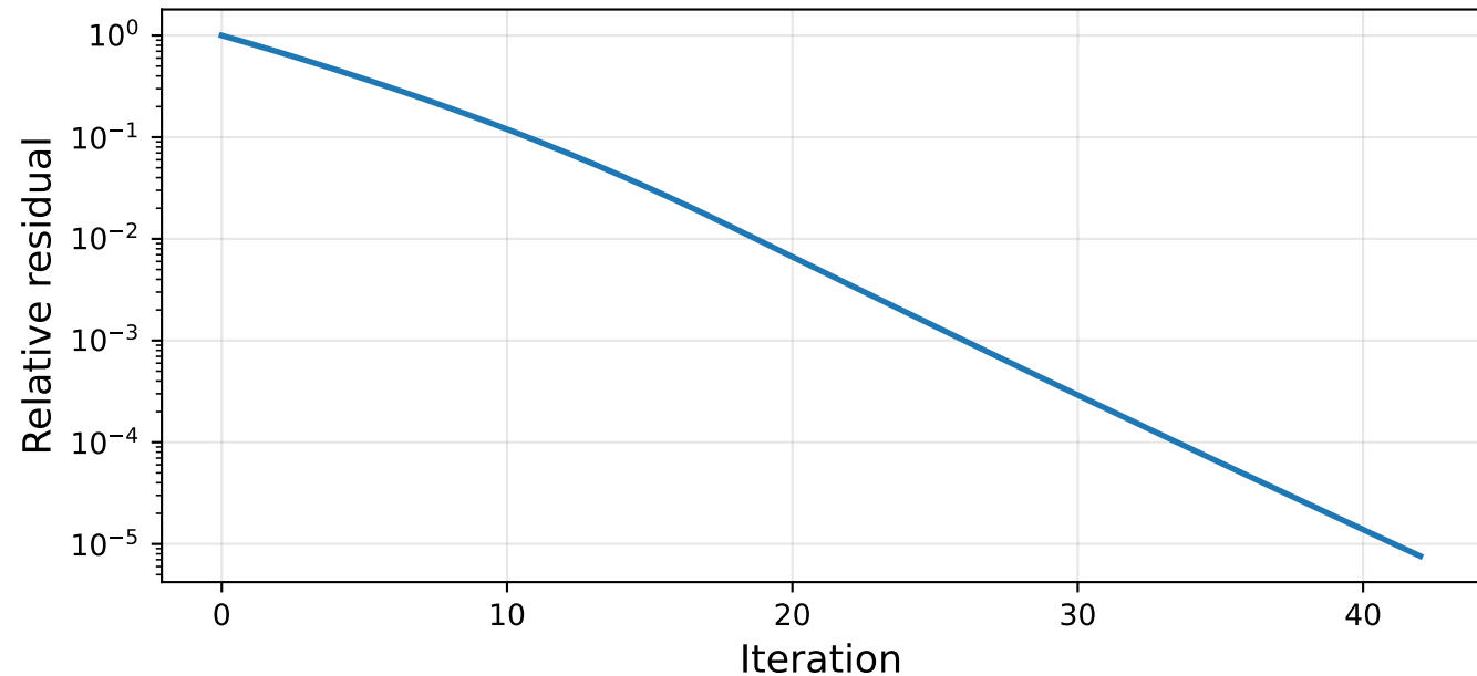
Outer Picard Residual
