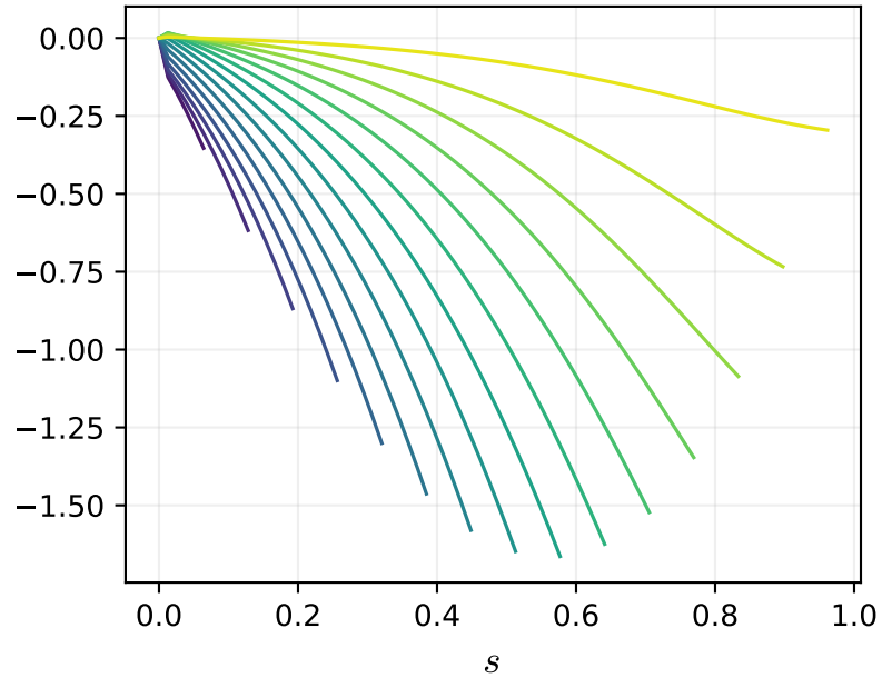
\mathcal{D}^1 channel W^1 \max|.|=1.66
