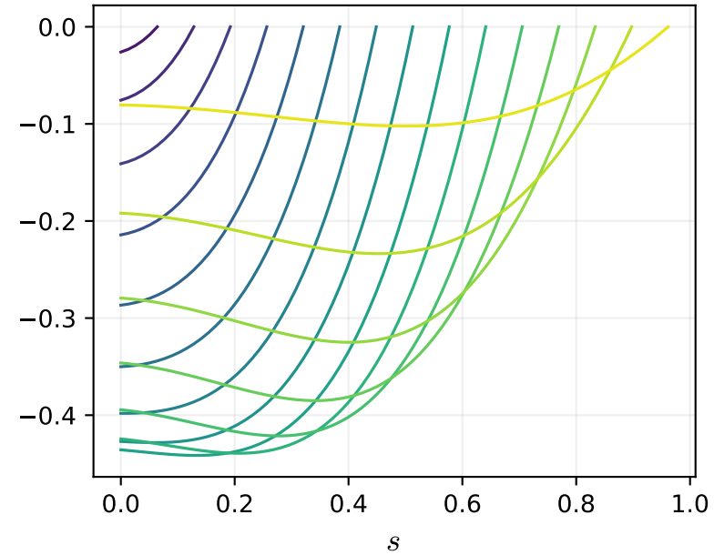
\mathcal{D}^1 channel W^0 \max|.|=0.442
