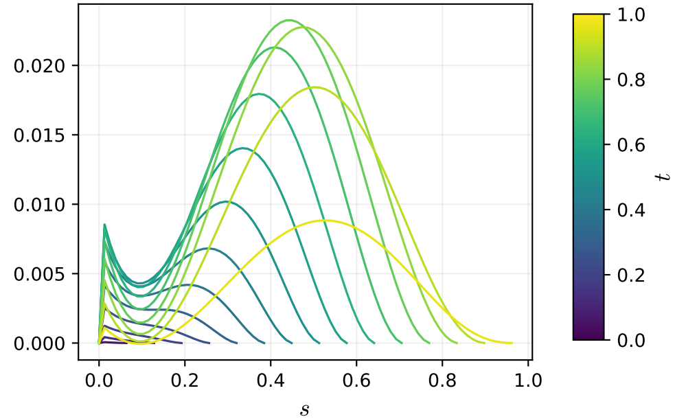
\mathcal{D}^1 channel W^2 \max|.|=0.0234
