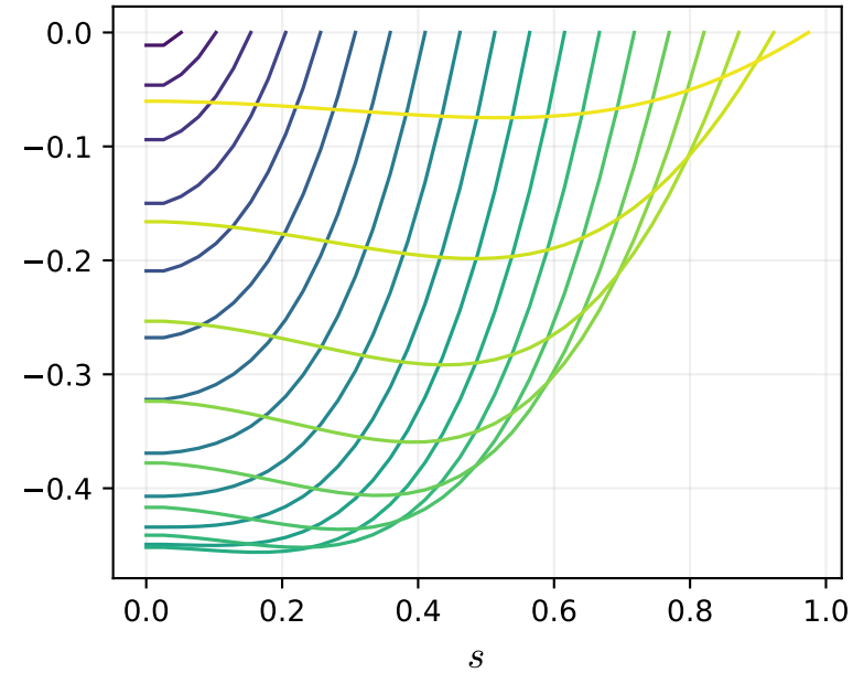
D^1 channel W^0 \max|.|=0.456
