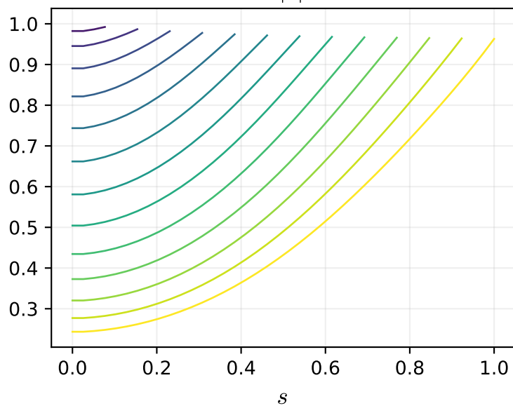
R^2 channel W^0 \max|.|=1
