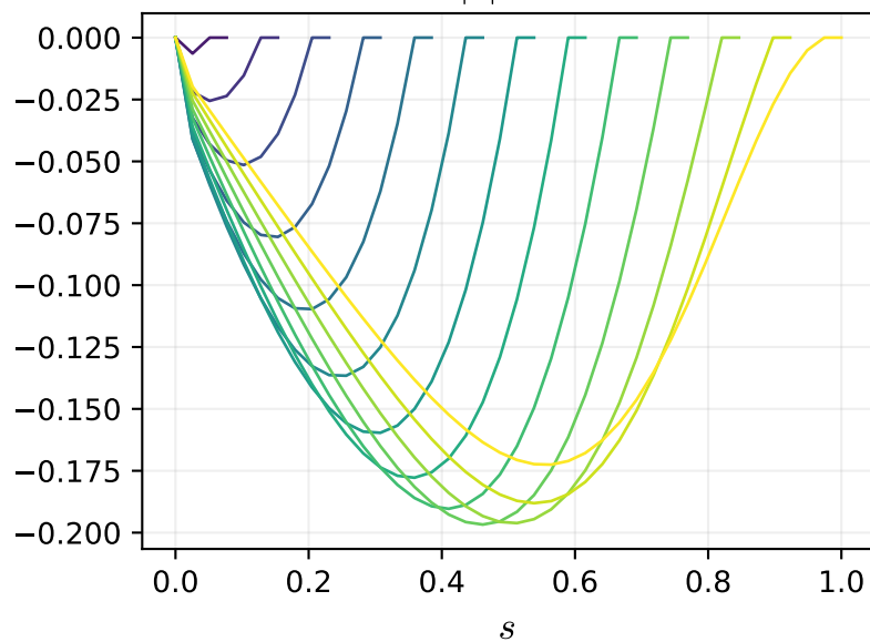
R^2 channel W^1 \max|.|=0.197
