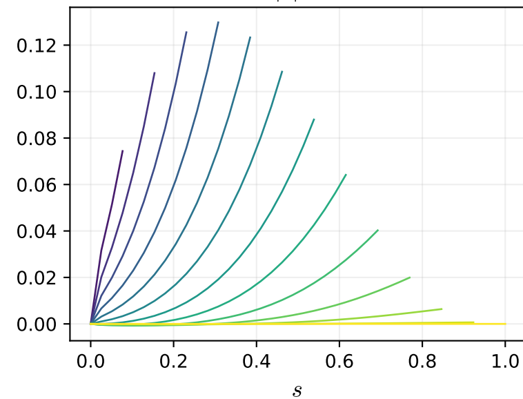
\bar{H}^2 channel W^2 \max|.|=0.13
