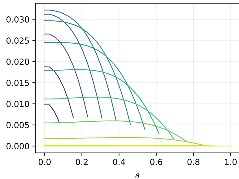
\bar{H}^2 channel W^0 \max|.|=0.0323
