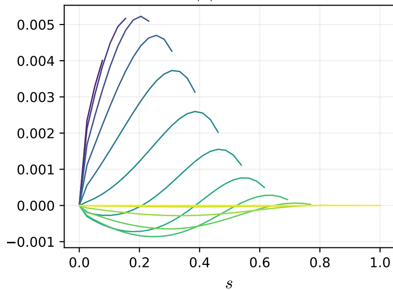
\bar{H}^2 channel W^1 \max|.|=0.00526
