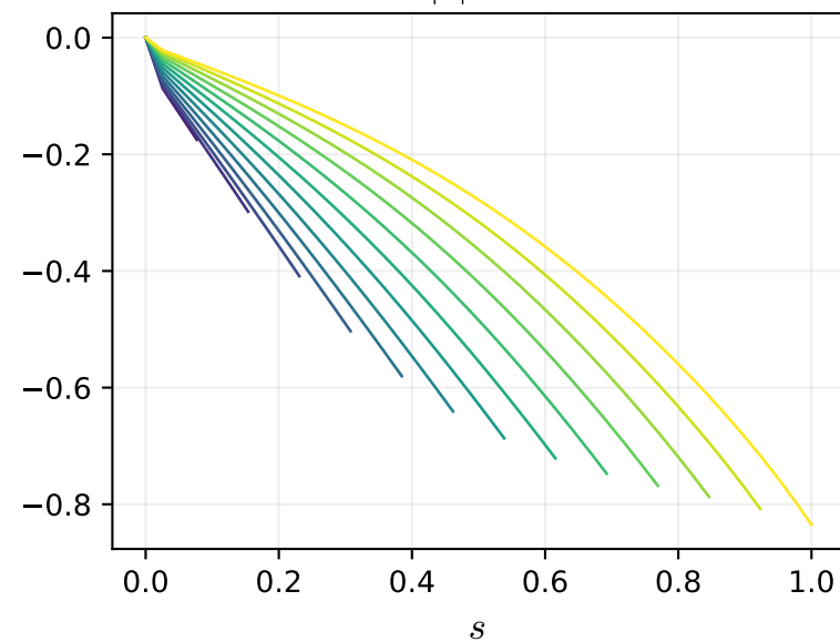
R^2 channel W^2 \max|.|=0.835
