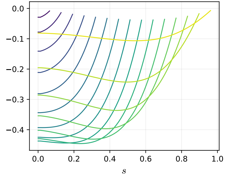
\mathcal{D}^1 channel W^0 \max|.|=0.447
