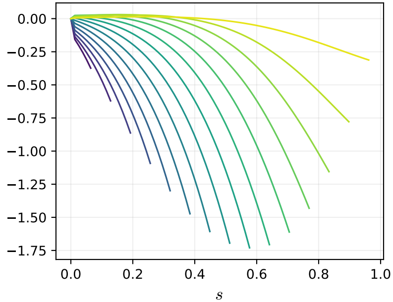
\mathcal{D}^1 channel W^1 \max|.|=1.73
