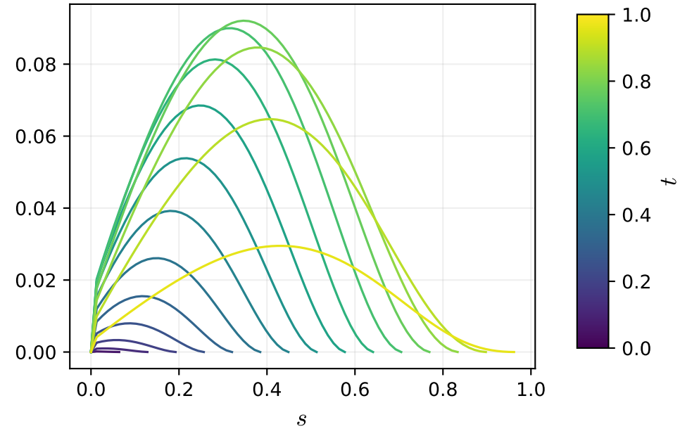
\mathcal{D}^1 channel W^2 \max|.|=0.0923
