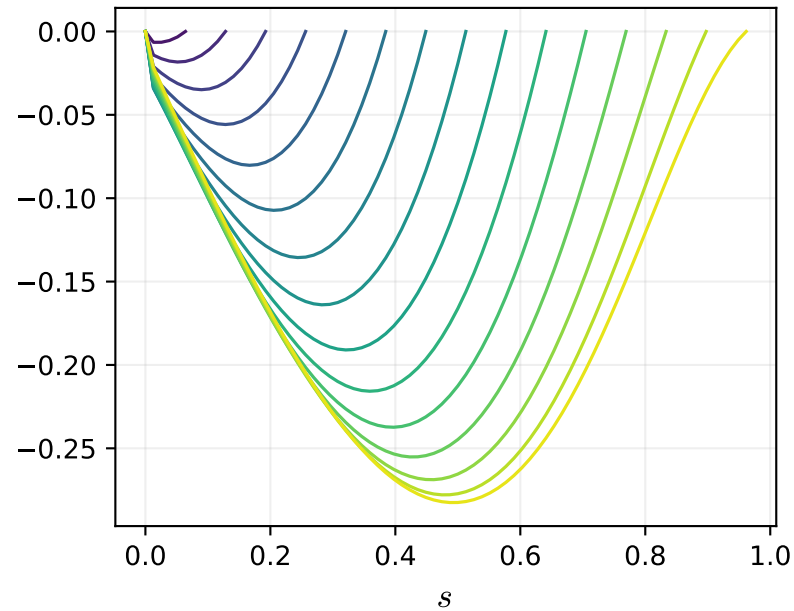
X channel W^1 \max|.|=0.283
