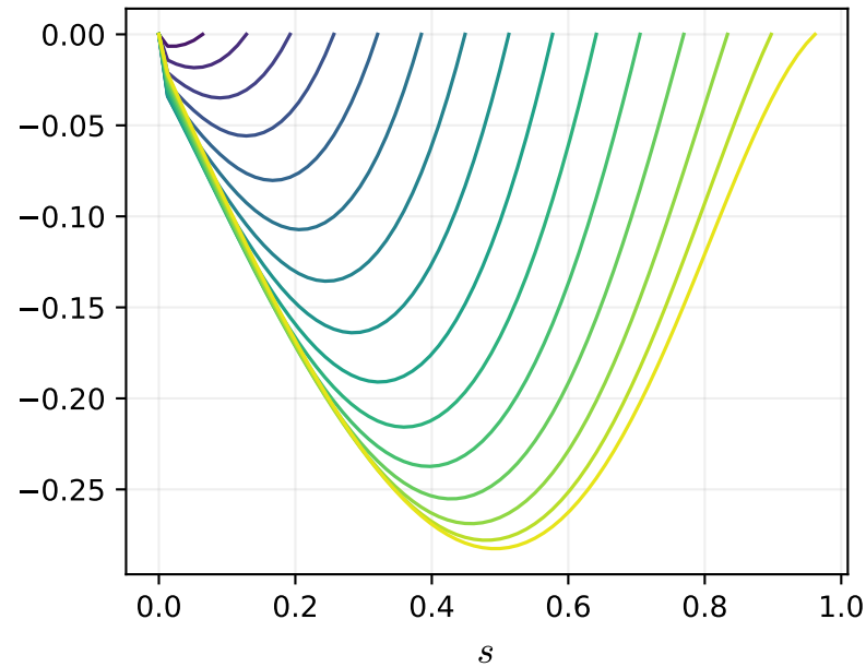
X channel W^2 \max|.|=0.283
