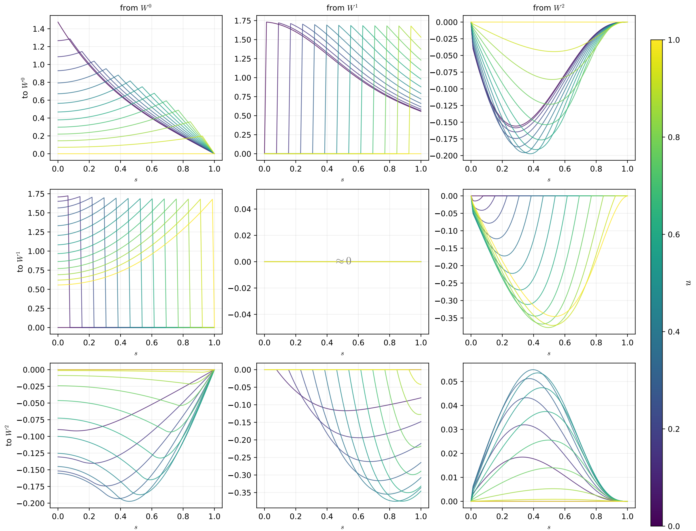
F^1 : entry slices of F_t(u, s) at t = T (color = u )
