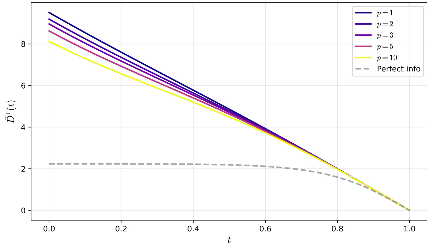
Player 1 mean control path \bar{D}^1(t) vs perfect info (color = p )
