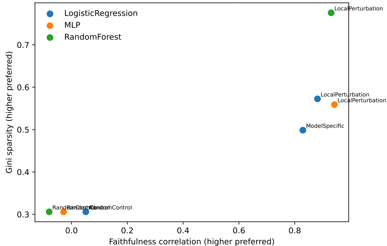
Measured benchmark trade-off; interpret with controls
