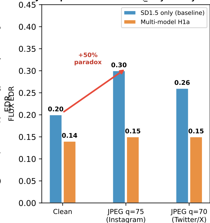
(c) JPEG Paradox on FLUX.1-schnell JPEG q=75 increases sd15\_only EDR by 50%
