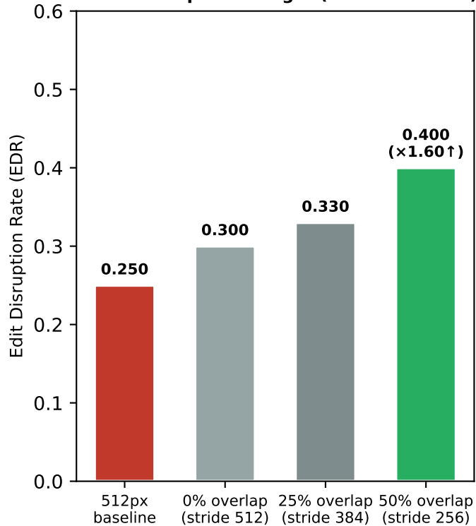
(a) Patch-Based High-Res Inference More overlap \rightarrow stronger ( \times 1.60 baseline)
