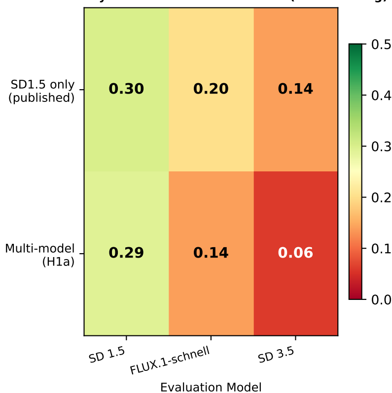
(b) Cross-Architecture Transfer SD1.5-only transfers to FLUX & SD3.5 (no retraining)
