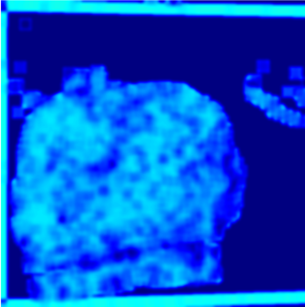
Singular Points
