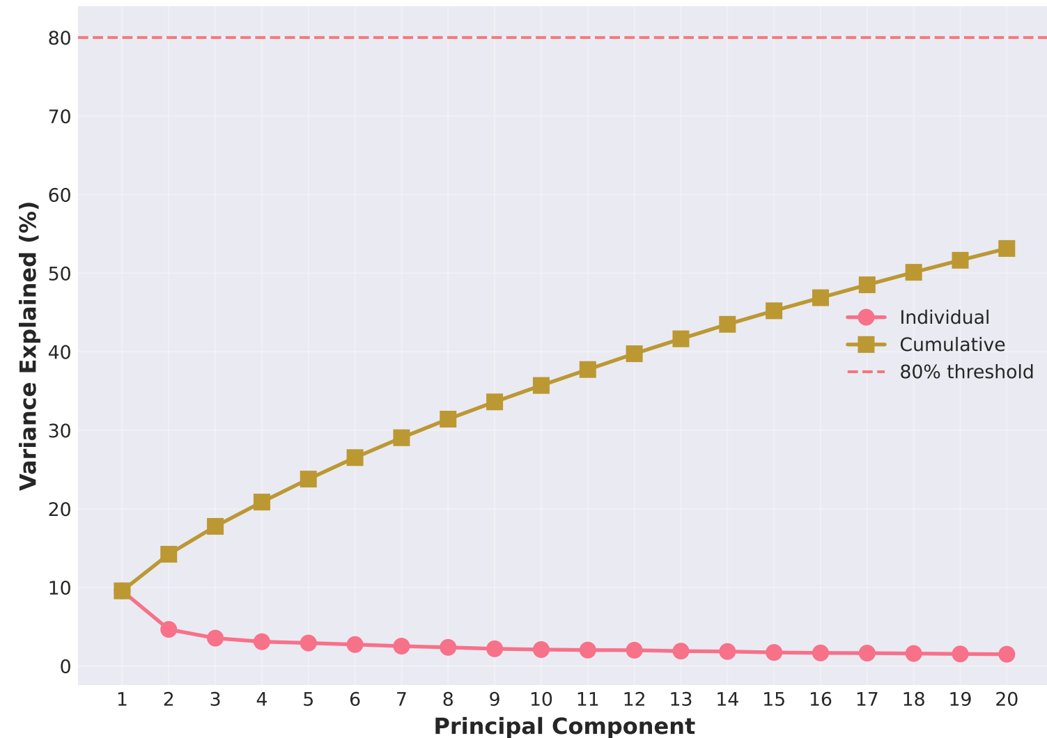
Scree Plot
