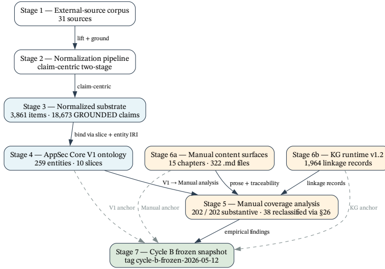
Figure 1: Pipeline Primitive Architecture. External-source corpus (31 sources) is normalized via the claim-centric two-stage pipeline into the normalized substrate (3,861 items, 18,673 GROUNDED claims). The normalized substrate binds against the AppSec Core V1 ontology (259 entities across 10 slices). The Manual coverage-analysis stage classifies per-entity Manual coverage and routes closure through three mechanisms (Section 6). Manual content surfaces and the KG runtime v1.2 (1,964 linkage records) are deposited at the cycle’s closure state cycle-b-frozen-2026-05-12 (Section 11).
