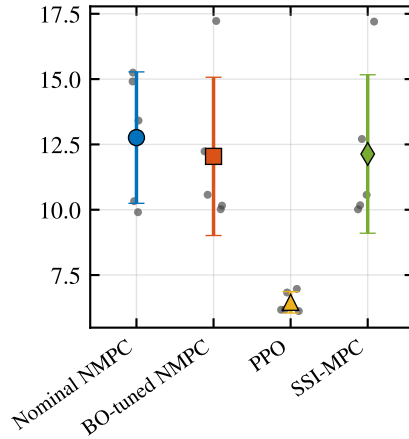
wall_dist_err_cm
