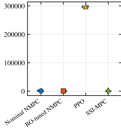
score.objective
