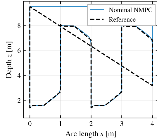
Nominal NMPC
