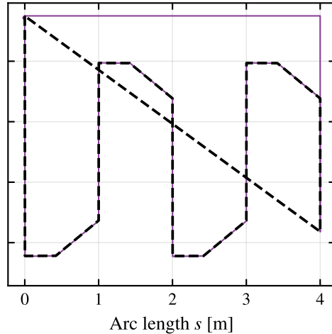
Diff-WMPC (ours)
