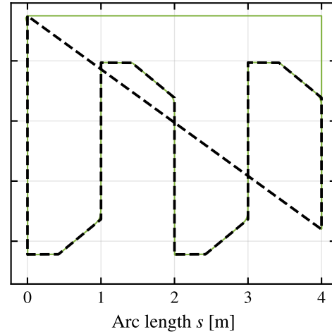
SSI-MPC
