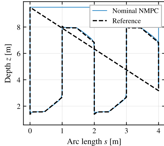
Nominal NMPC
