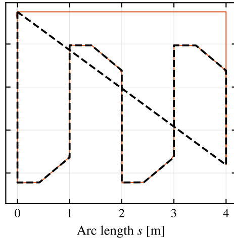
BO-tuned NMPC
