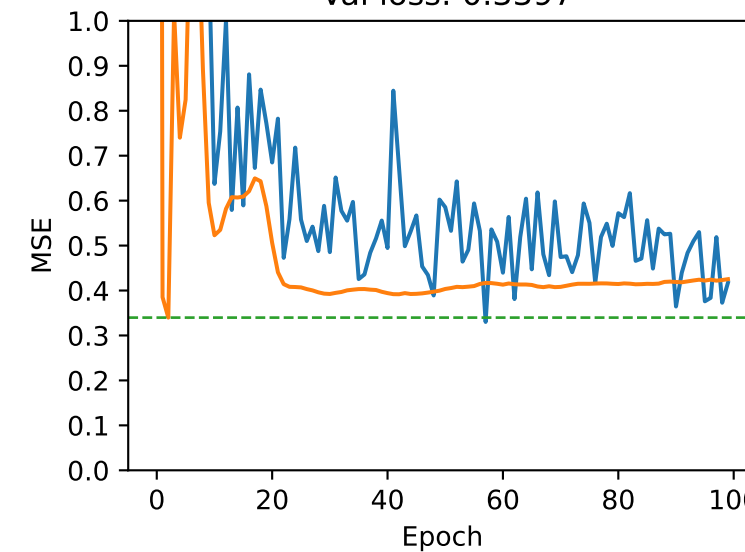
Top model 10 Val loss: 0.3397
