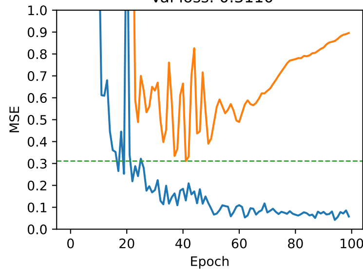
Top model 6 Val loss: 0.3110
