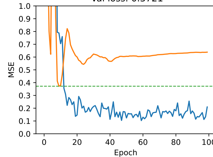
Top model 9 Val loss: 0.3721
