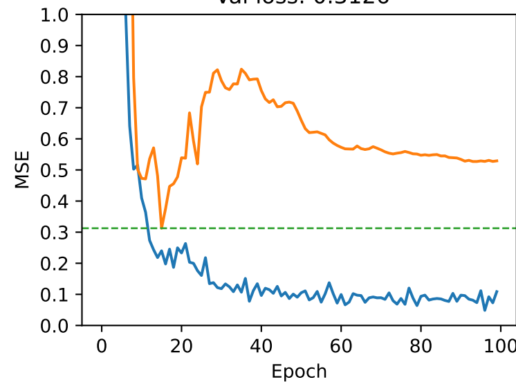
Top model 7 Val loss: 0.3126
