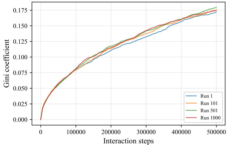
Sample paths: same rules, different luck
