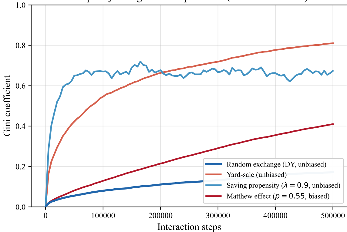
Inequality emerges from equal starts (DY needs no bias)
