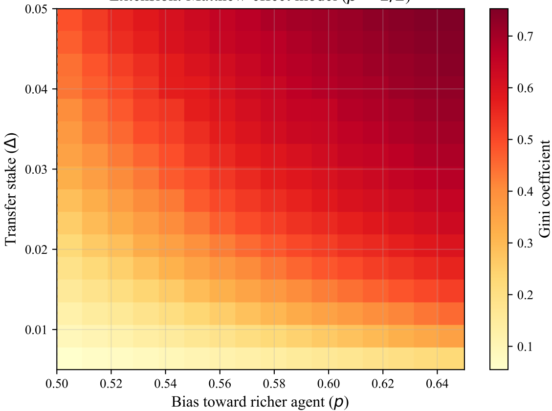
Extension: Matthew-effect model ( p > 1/2 )
