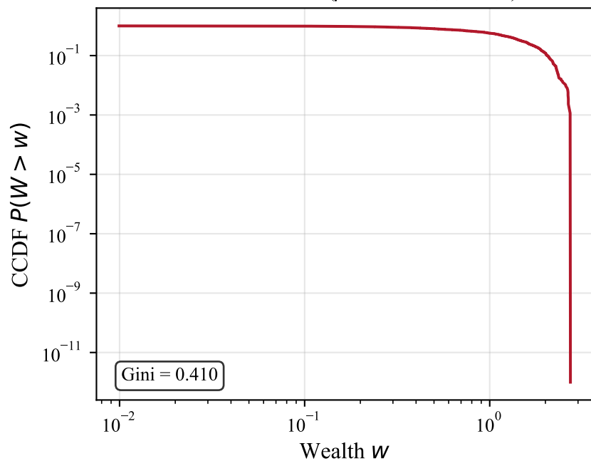
Matthew effect ( p = 0.55 , biased)
