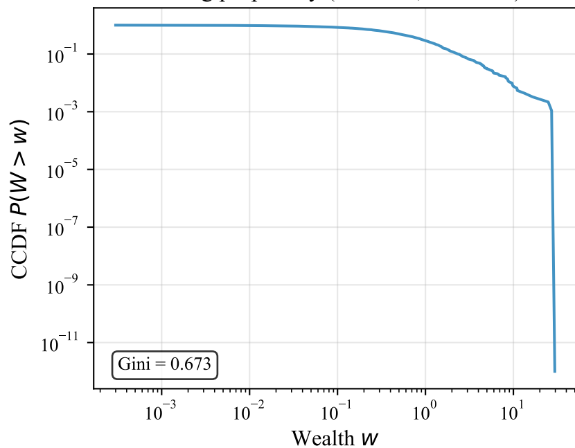
Saving propensity ( \lambda = 0.9 , unbiased)
