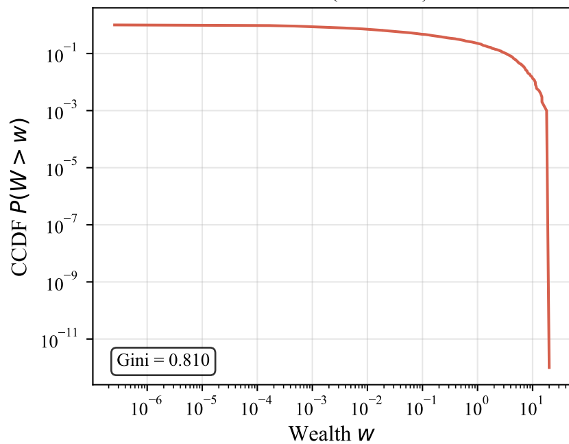
Yard-sale (unbiased)
