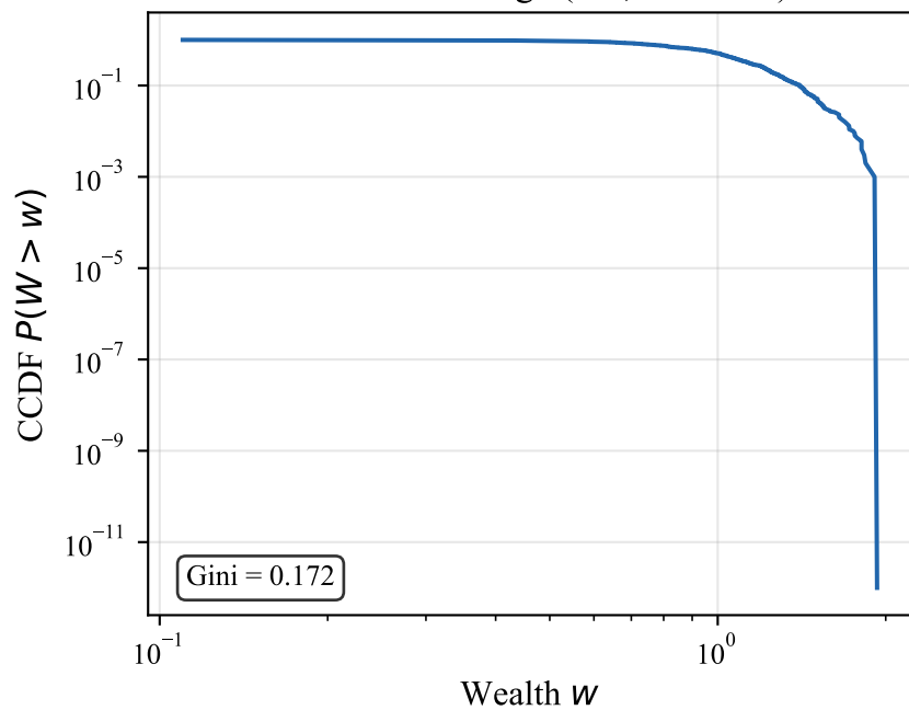
Random exchange (DY, unbiased)
