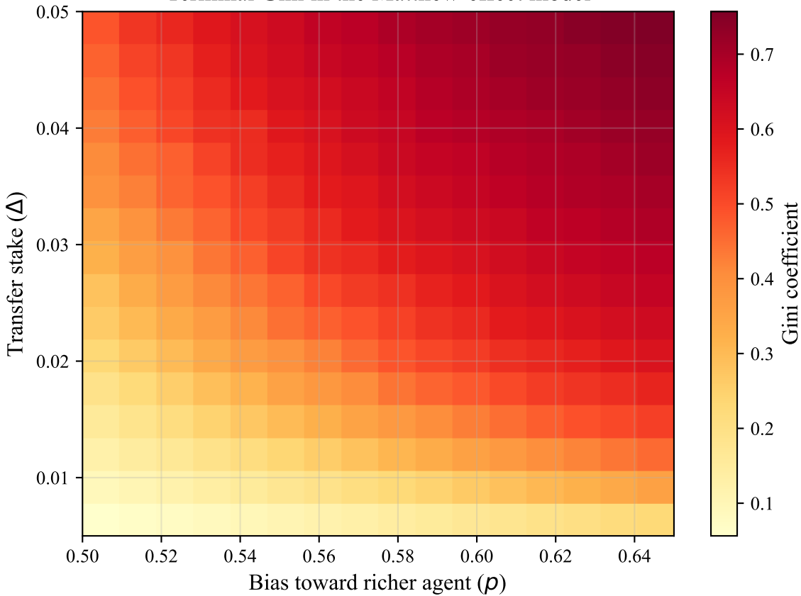
Terminal Gini in the Matthew-effect model
