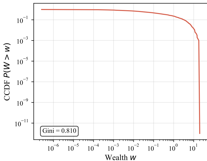
Yard-sale
