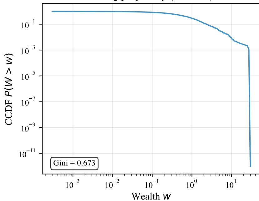
Saving propensity ( \lambda = 0.9 )
