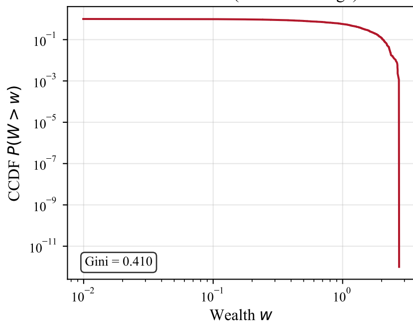
Matthew effect (biased exchange)
