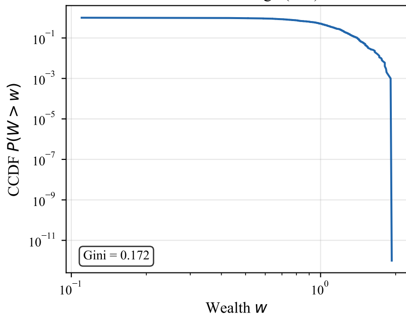
Random exchange (DY)
