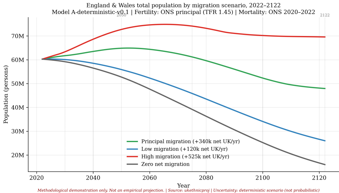
Figure 1: Total England and Wales population under four ONS 2022-based migration scenarios, 2022–2122. Fertility and mortality held constant; migration is the only varying input. Conditional projection only; not a forecast.
