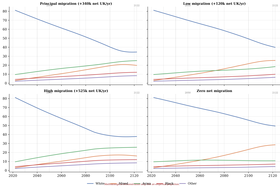
Figure 4: Ethnic composition in England by migration scenario (small multiples), 2022–2122. Each panel shows the same five ethnic groups under a different ONS migration variant.
