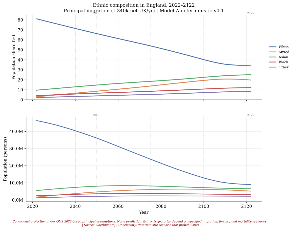
Figure 3: Ethnic population shares and counts in England under the principal ONS 2022-based migration variant (Census 2021 base, mid-2022), 2022–2122. Wales is included in population totals but excluded from share panels. Conditional projection only; not a forecast.
