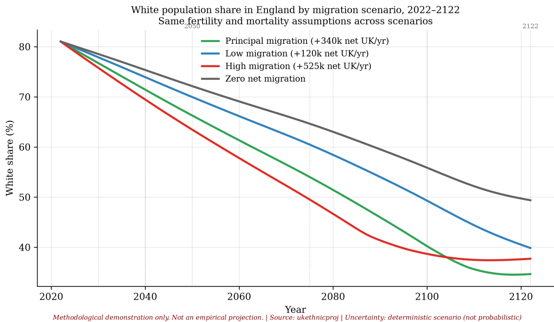
Figure 2: White population share in England under four migration scenarios, 2022–2122. Higher net migration produces faster diversification of ethnic composition under the calibrated parameter set.
