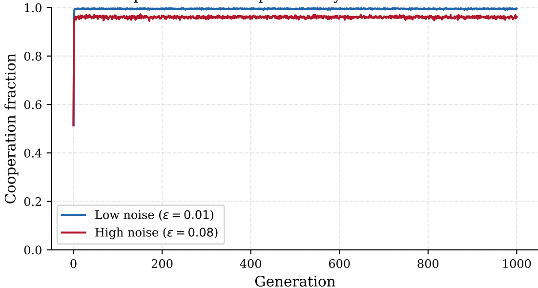
Spatial model: cooperation dynamics over time
