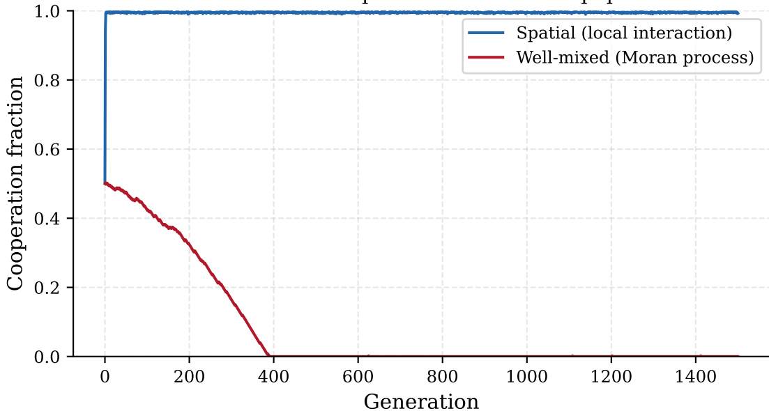
Structure matters: spatial vs. well-mixed population
