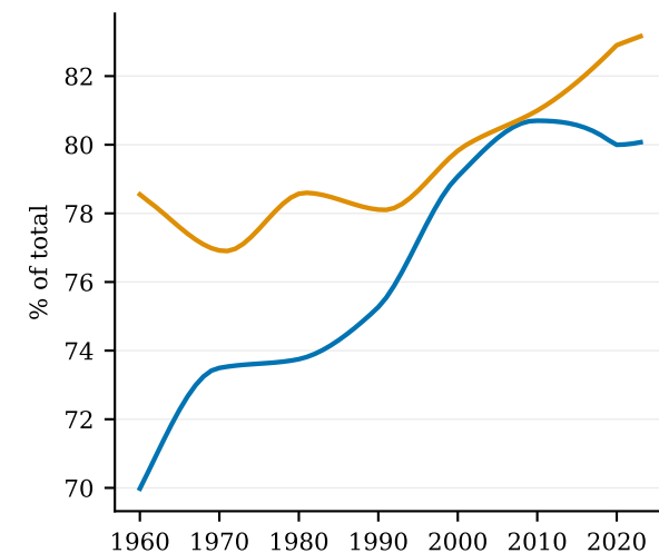
Urbanisation share
