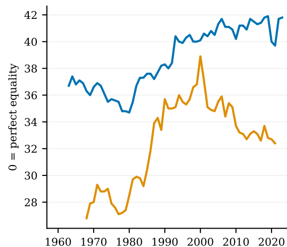
Gini index
