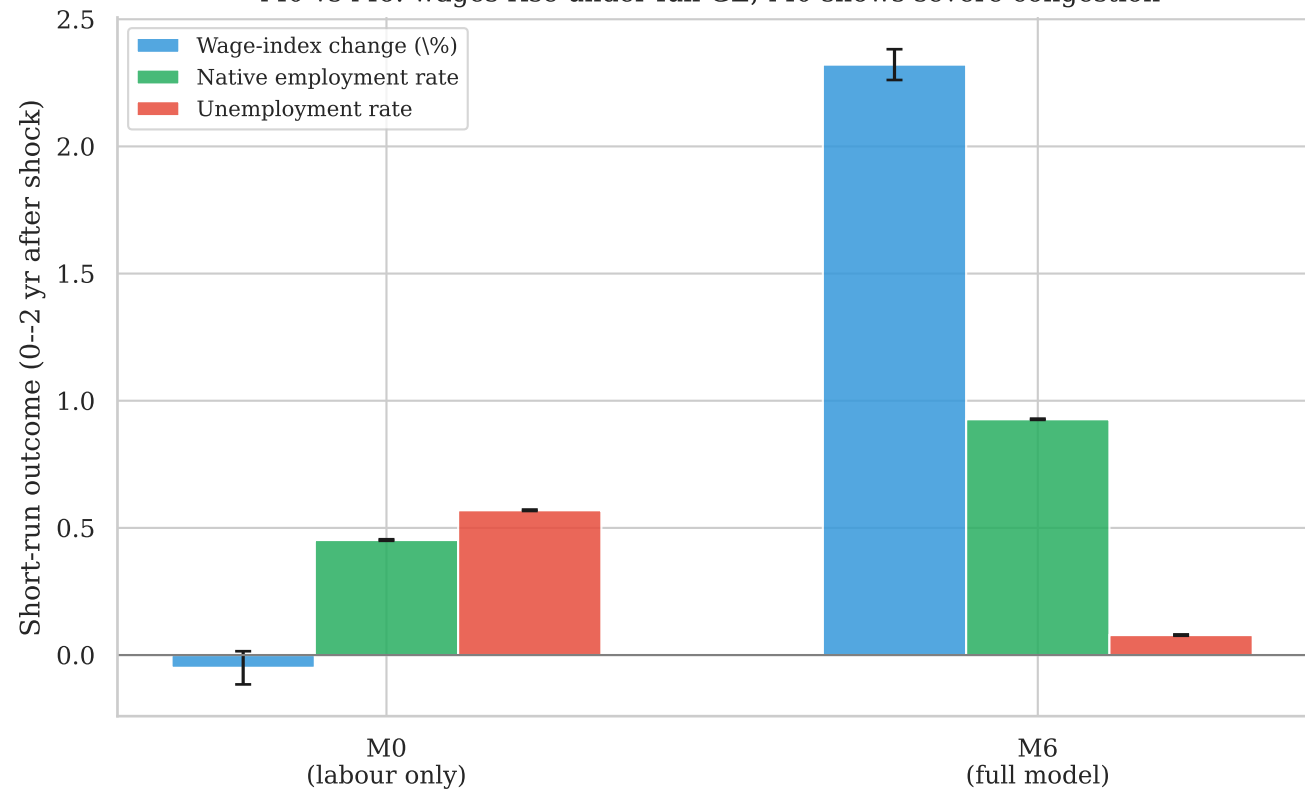
M0 vs M6: wages rise under full GE; M0 shows severe congestion
