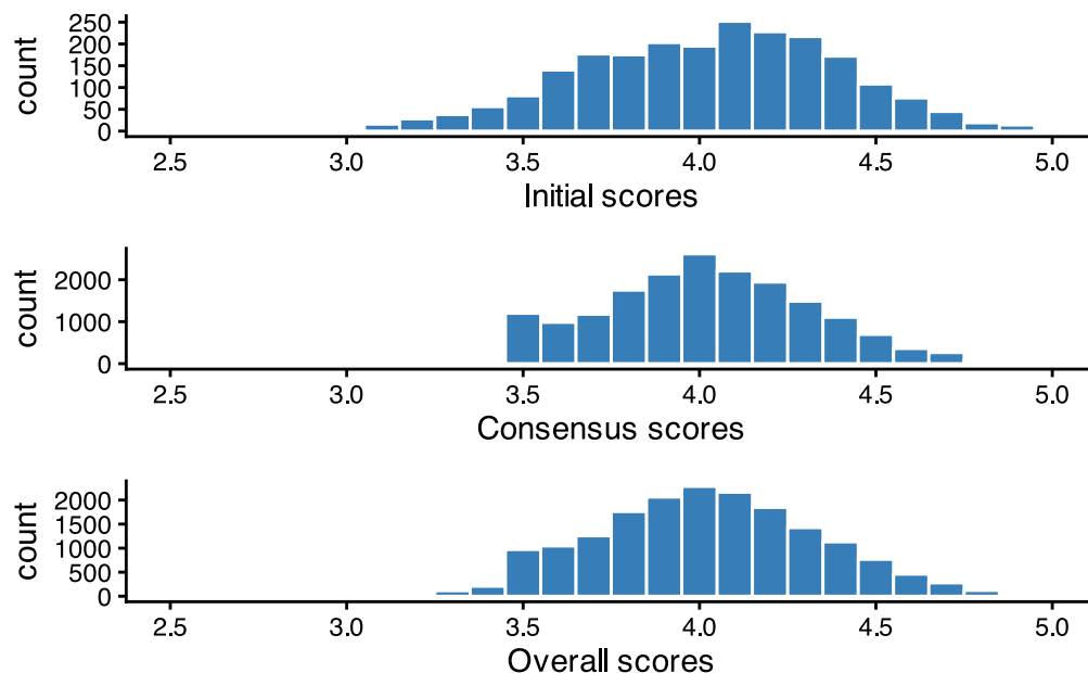
Figure 1: Distribution of simulated intial, consensus, and overall scores
