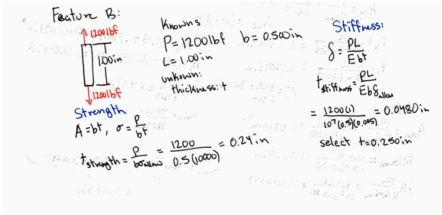
Original handwritten B strength and stiffness calculations. .
