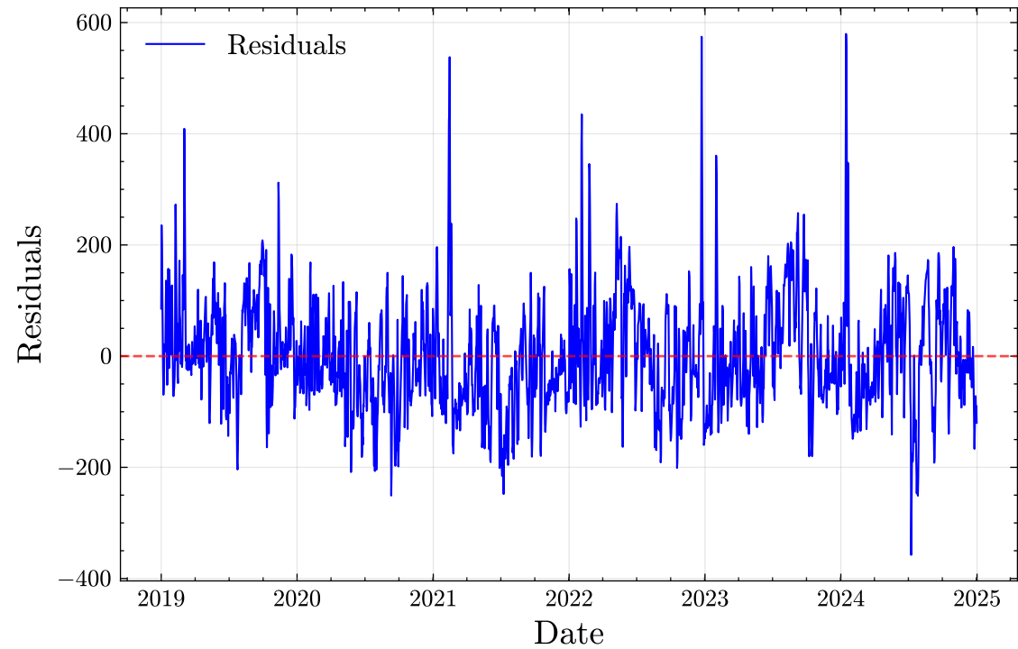
Residuals
