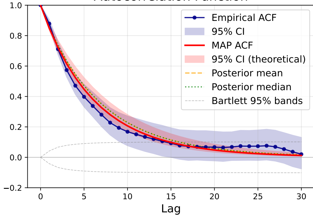
Autocorrelation Function
