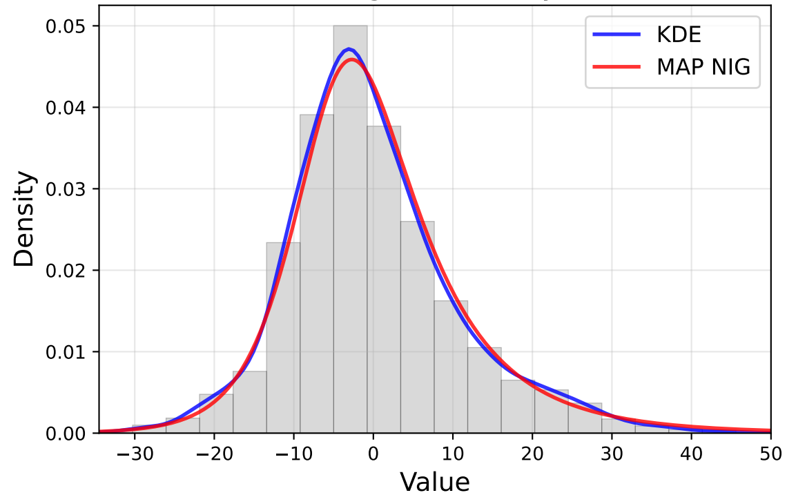
Marginal Density
