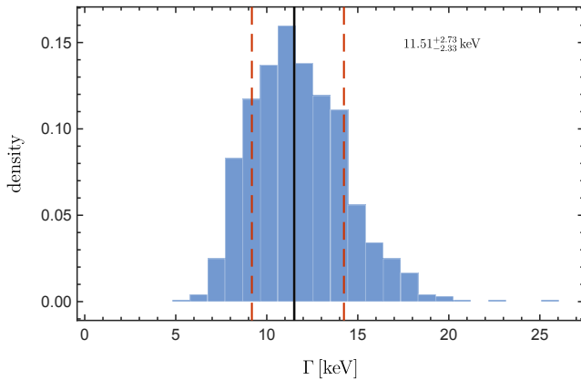
B_{s1}(5750) \rightarrow B_s \gamma
