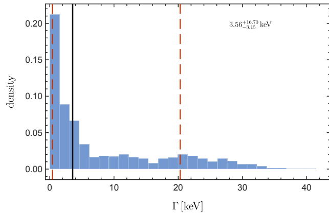
B_{s1}(5830) \rightarrow B_s \gamma
