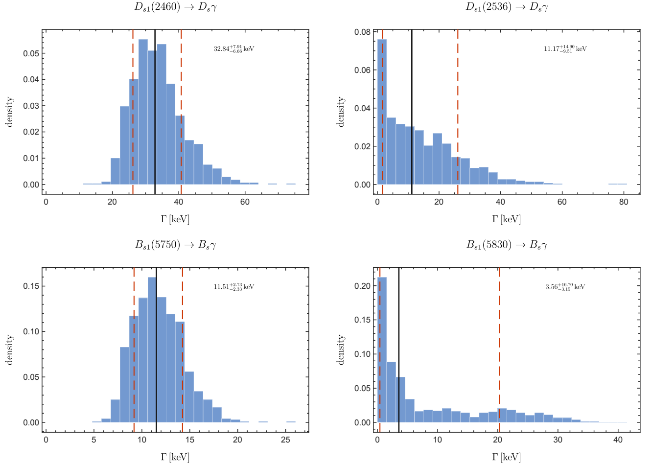
FIG. 3: Monte Carlo distributions of the radiative decay widths from the broad 25^\circ \leq \theta \leq 45^\circ sensitivity scan. The solid and dashed vertical lines indicate the median and the 16th–84th percentile interval, respectively. These benchmark distributions are not used for the preferred final uncertainties.
