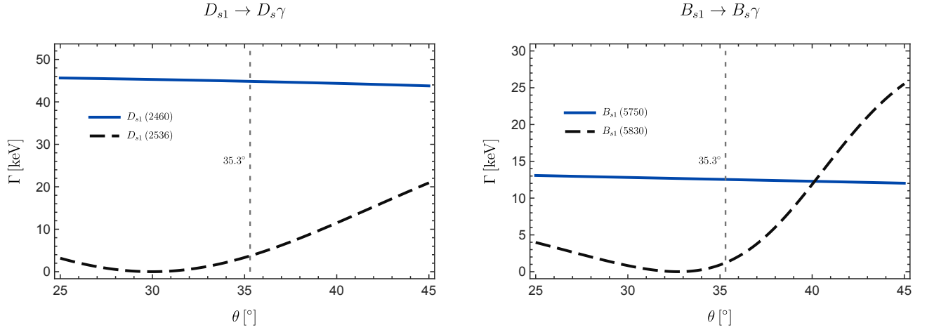
FIG. 2: Dependence of the radiative decay widths on the mixing angle \theta . The charm-strange and bottom-strange channels are shown in the left and right panels, respectively. The vertical dashed line marks \theta = 35.3^\circ , the heavy-quark-limit reference value. The 25^\circ – 45^\circ range is shown only as a sensitivity test.
