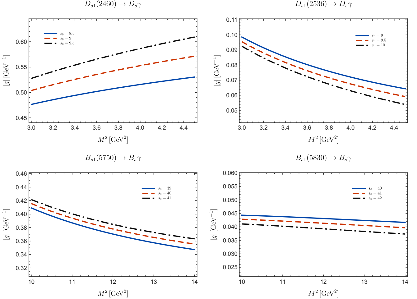
FIG. 1: Borel-parameter dependence of the transition form factors for D_{s1}(2460) \rightarrow D_s\gamma , D_{s1}(2536) \rightarrow D_s\gamma , B_{s1}(5750) \rightarrow B_s\gamma , and B_{s1}(5830) \rightarrow B_s\gamma . The curves correspond to representative values of the continuum threshold s_0 .
