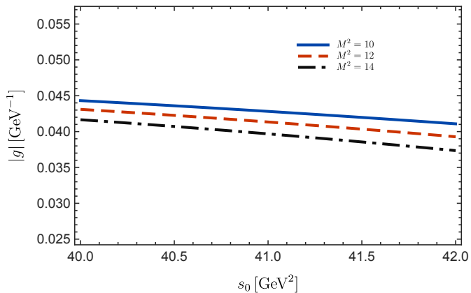
B_{s1}(5830) \rightarrow B_s \gamma
