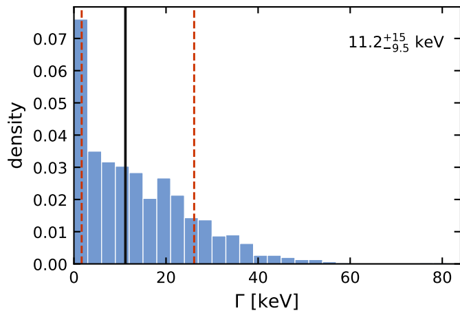
B_{s1}(5830) \rightarrow B_s \gamma
