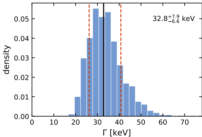
B_{s1}(5750) \rightarrow B_s \gamma
