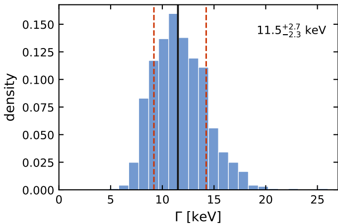
B_{s1}(5750) \rightarrow B_s \gamma
