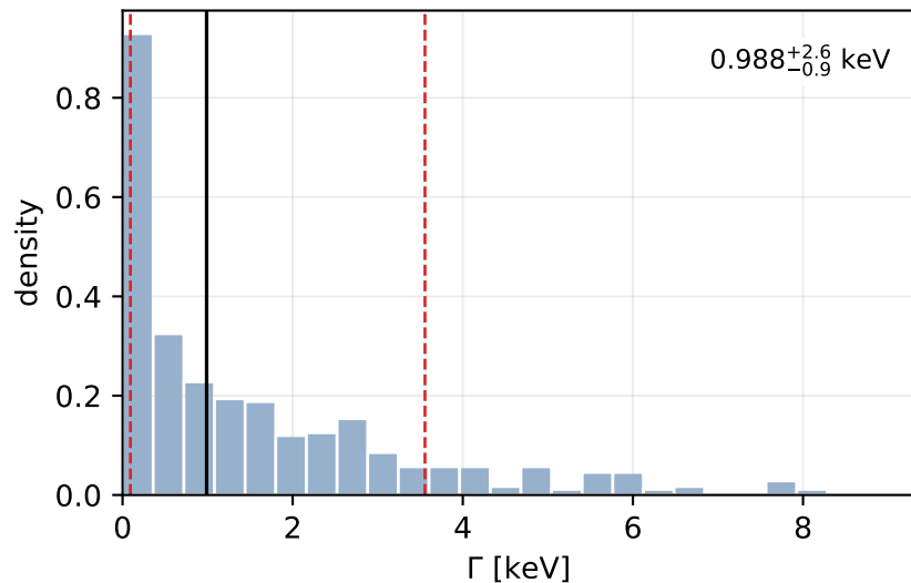
D_{s1}(2536) \rightarrow D_s \gamma
