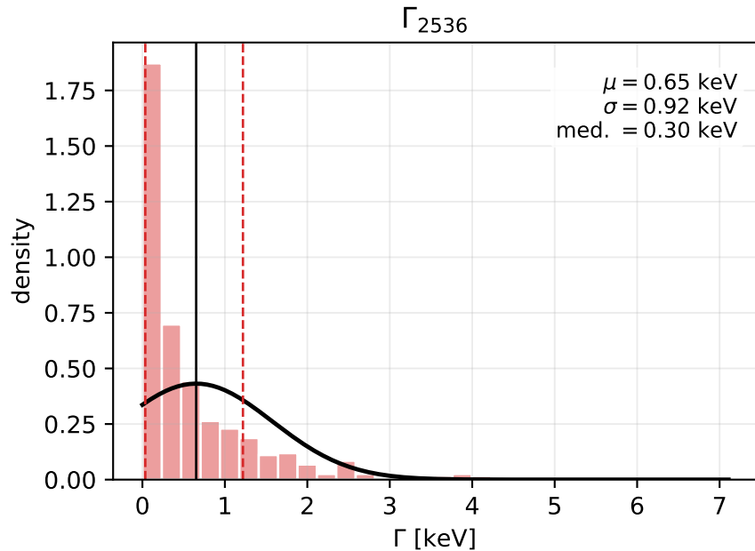
Lattice-normalized Monte Carlo width distribution, 25^\circ \leq \theta \leq 45^\circ
