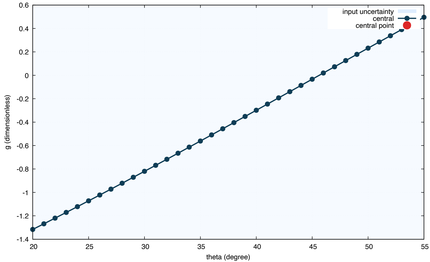
B_{s1}(5830) \rightarrow B_s^* \gamma ; mixing-angle sensitivity
